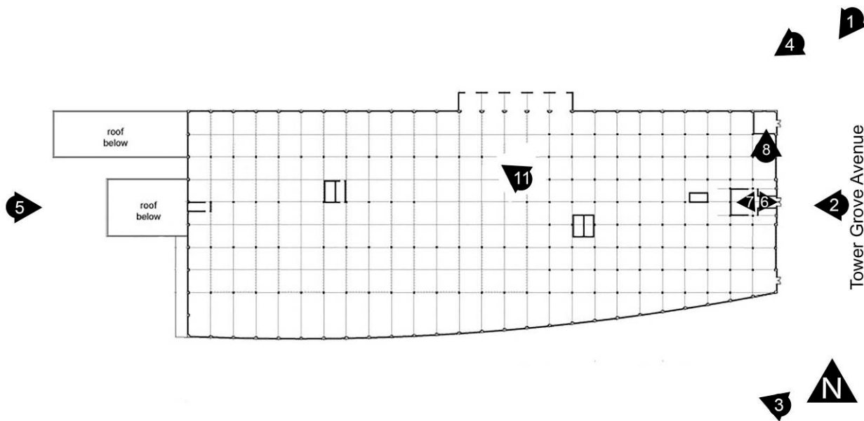
Figure 3: Woodward & Tiernan Printing Company Building, third floor plan. Source: Base plan provided by UIC/Urban Improvement Company.
