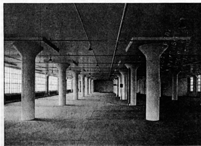
Interior of typical flat slab concrete building, showing use of gloss white paint to increase effective illumination. Tiffin Building, Long Island City, N. Y. The Ballinger Company, Architects and Engineers
