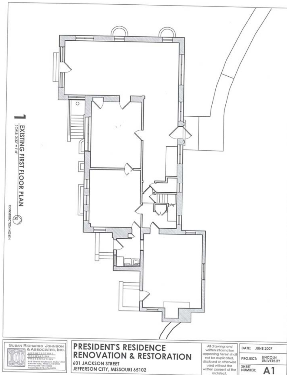
Figure 1: Floorplan
