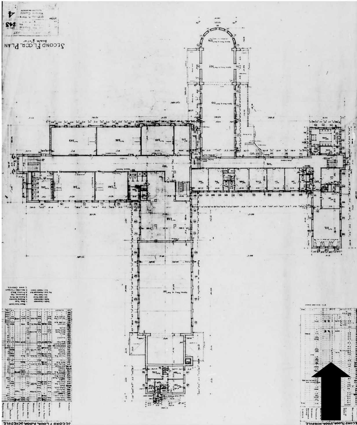
Figure 7. High School and Seminary Plan, second floor, 1930. Source: Carroll, Maurice and O'Meara & Hills Saint John's Seminary, original plans. March 1930.
