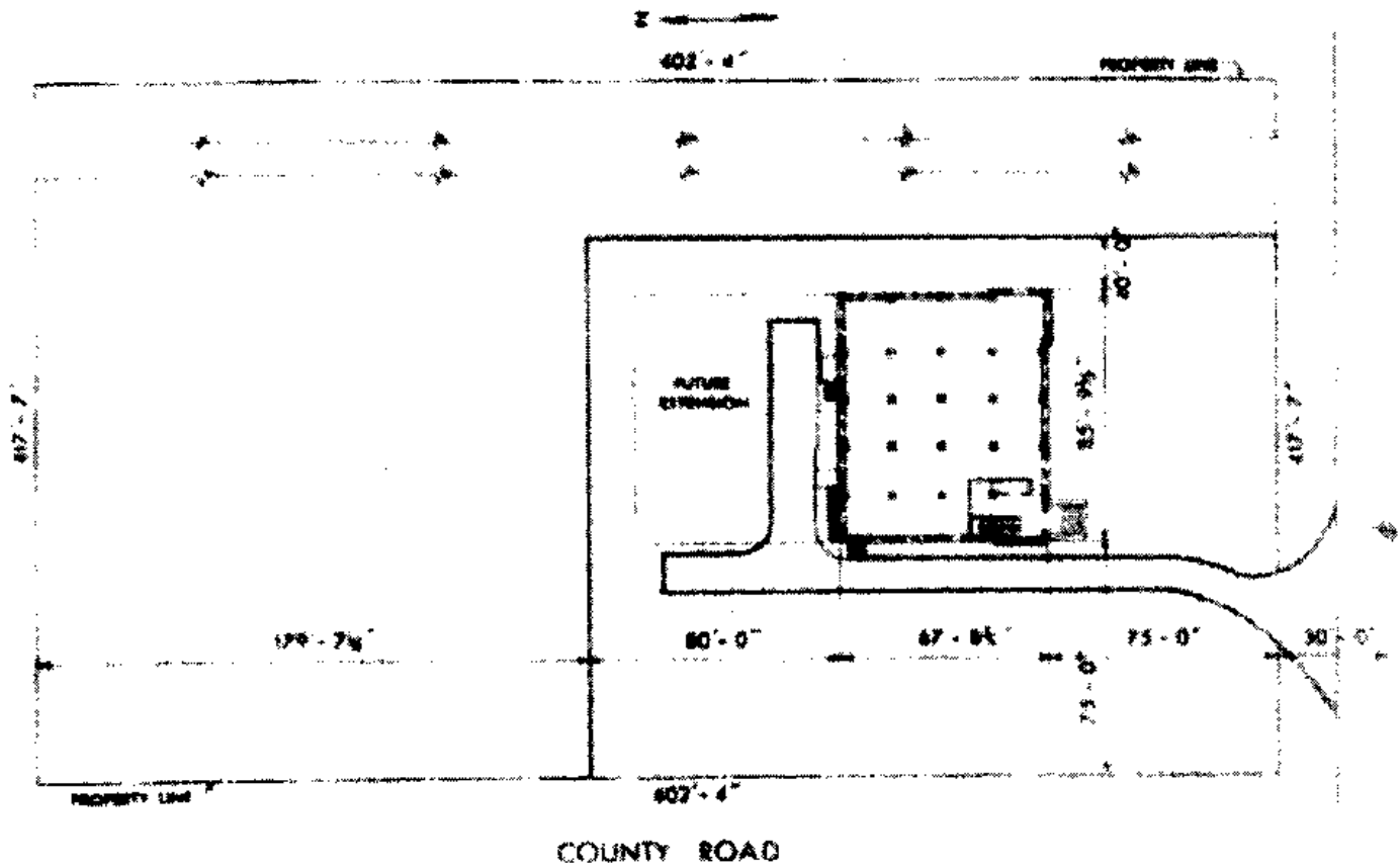
Figure 1: Site Plan of the Wright City Southwestern Bell Repeater Station. Source: AT&T Archives and History Center, San Antonio, Texas. General Building Data Sheets (4 pages), 1930. This site plan shows the property as it appeared in 1930; the site was reduced during the period of significance to comprise the present site boundary bound by the darker rectangle below.
