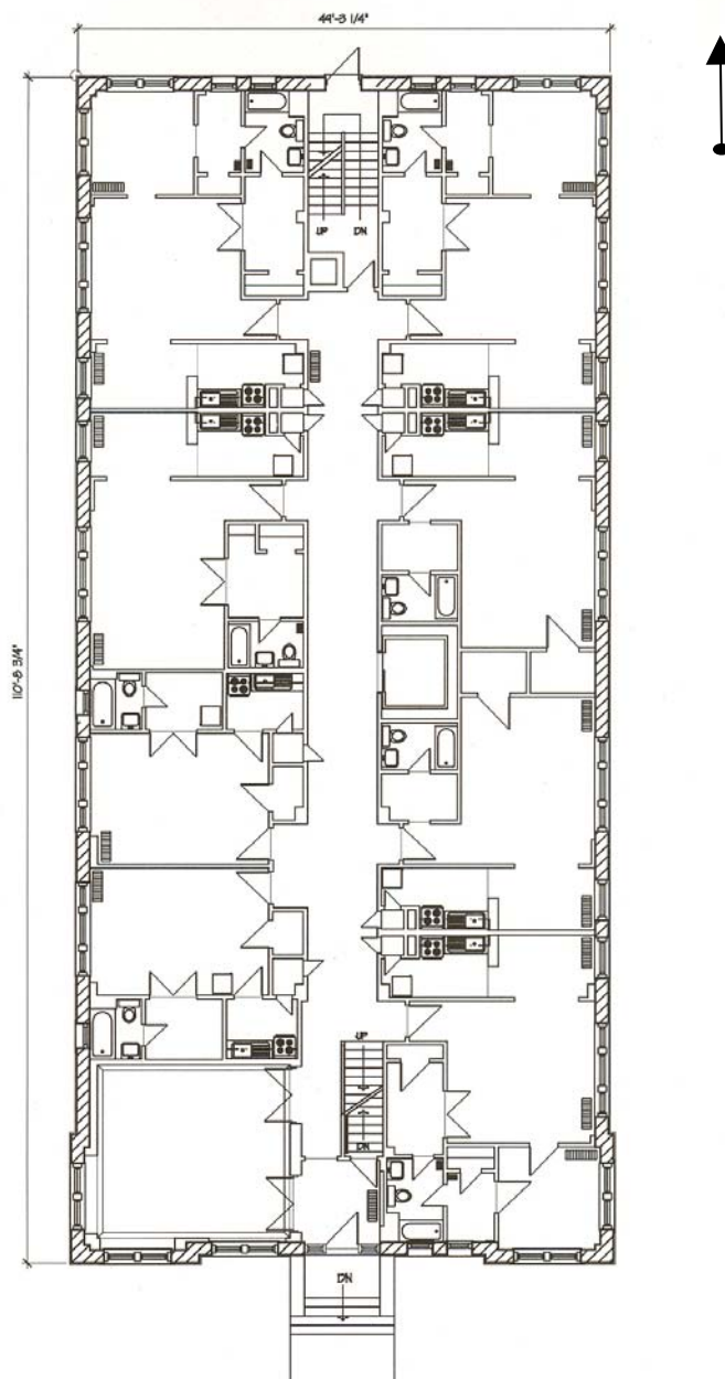
Figure Two. First Floor Plan. Plan courtesy of SWD Architects, Inc.
