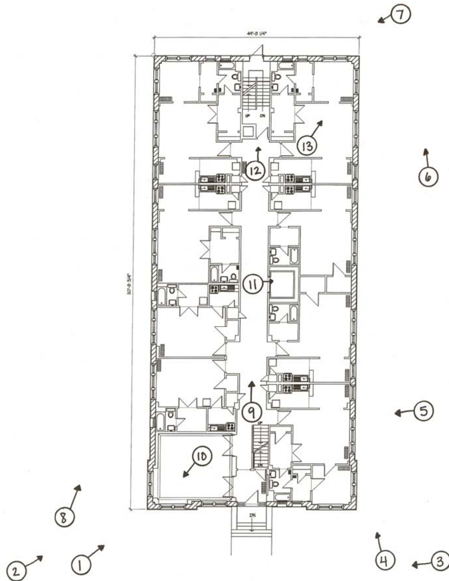
A4 FIRST FLOOR PLAN SCALE _____ NORTH
