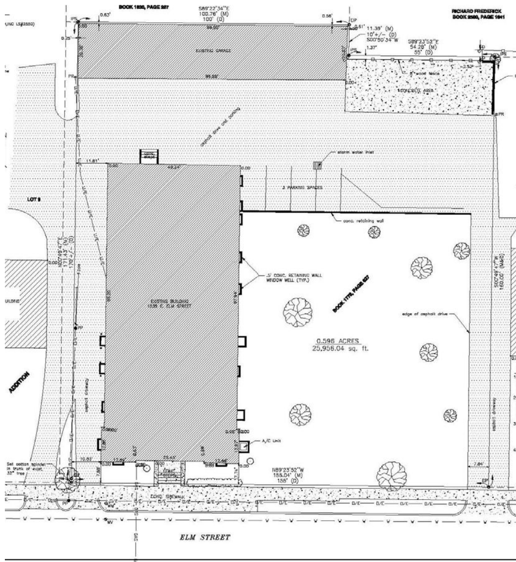
Figure One. Site Plan. Prepared by Hood-Rich Inc, Springfield, MO 12/31/07.
